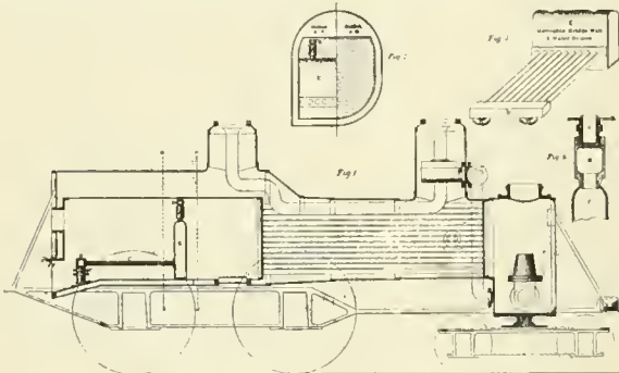
NORRIS' COAL BURNING BOILER. FIG. 69.
